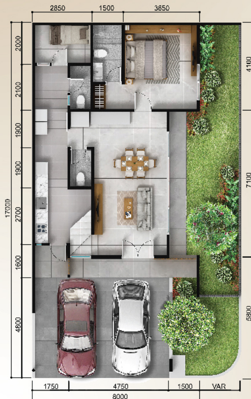
Lantai 1
