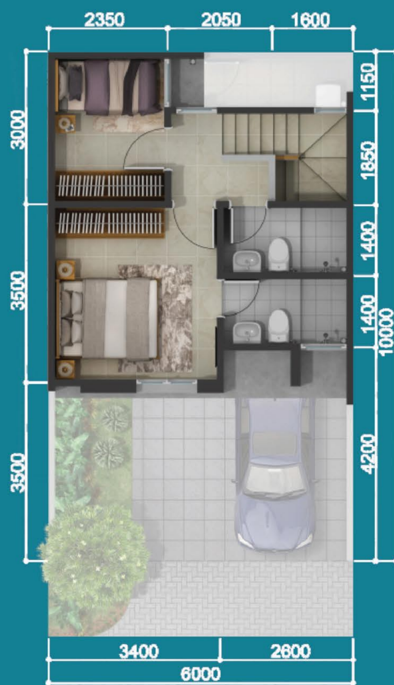
Denah Lantai 2
