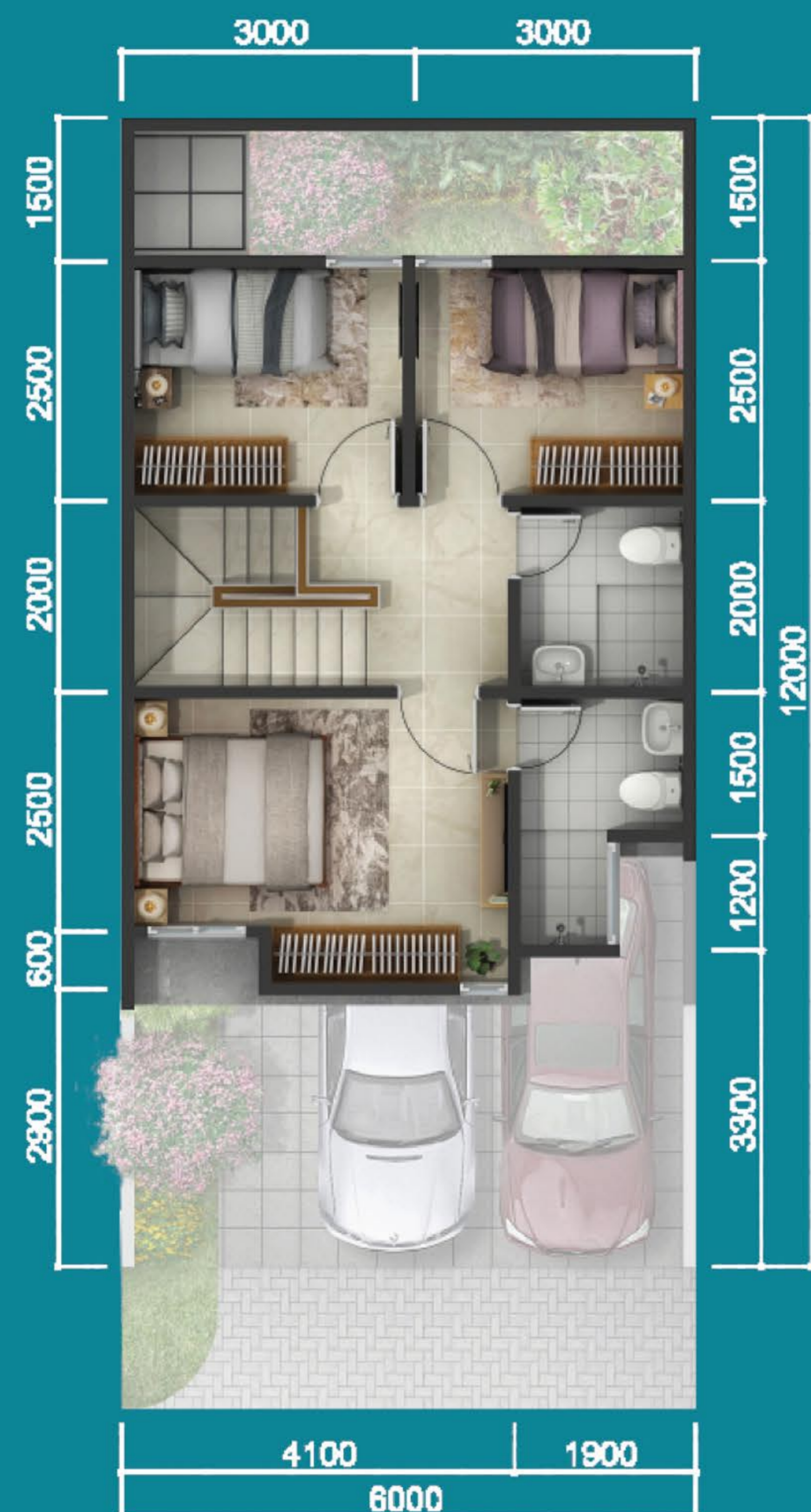
Denah Lantai 2
