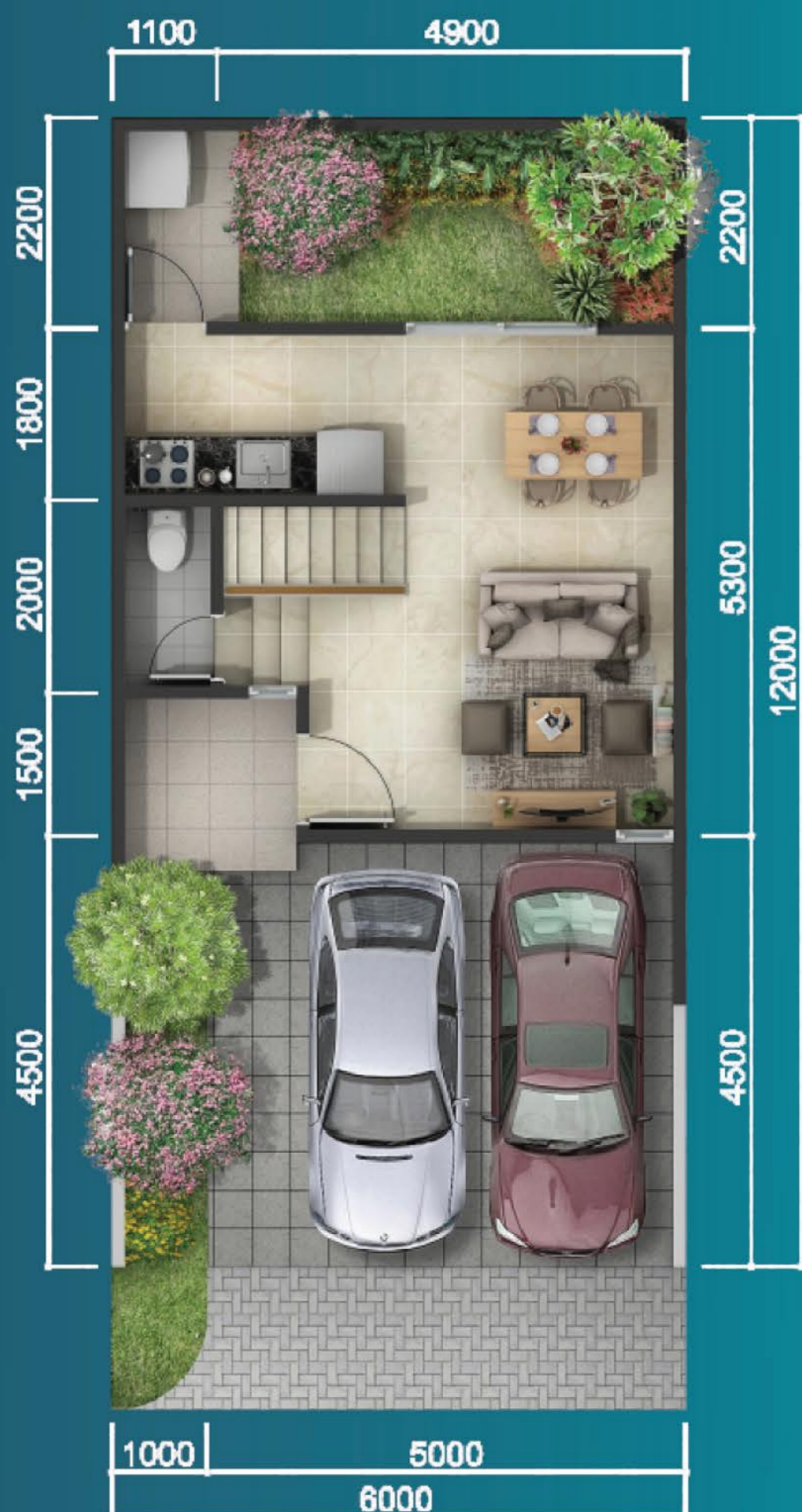
Denah Lantai 1
