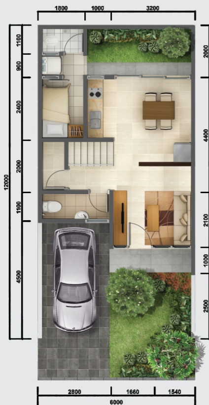
Denah Lantai 1
